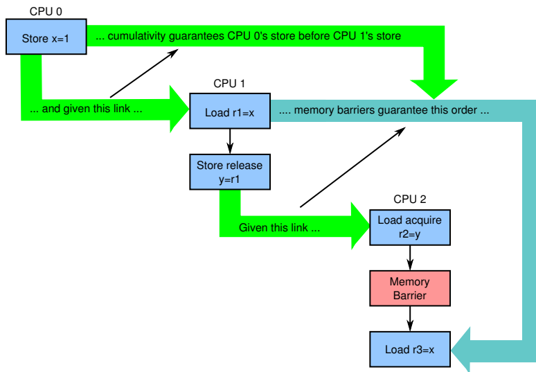
Figure 15.9: Cumulativeness
