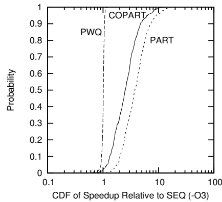
Figure 6.30: Partitioned Coroutines
