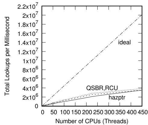
Figure 10.8: Read-Only RCU-Protected Hash-Table Performance For Schrödinger's Zoo including QSB, Linear Scale
