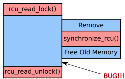
Figure 9.14: Summary of RCU Grace-Period Ordering Guarantees
