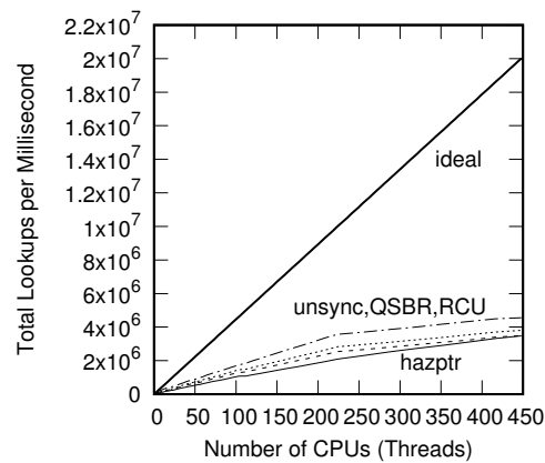
Figure 10.9: Read-Only RCU-Protected Hash-Table Performance For Schrödinger's Zoo including QSB and Unsynchronized, Linear Scale
