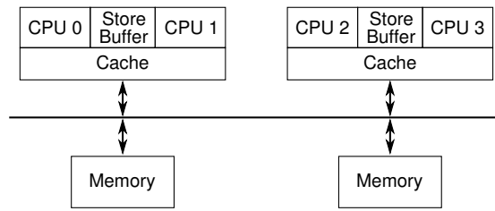
Figure 15.8: Shared Store Buffers And Multi-Copy Atomicity
