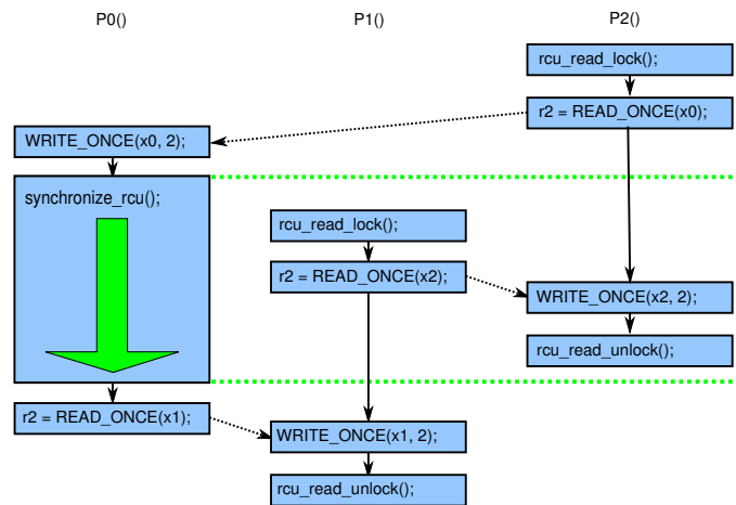
Figure 15.14: Cycle for One RCU Grace Period and Two RCU Readers
