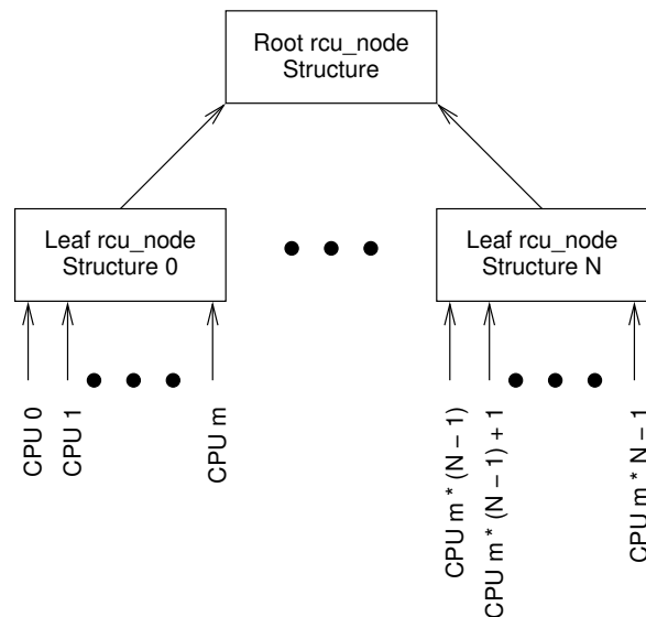
Figure 7.9: Locking Hierarchy
