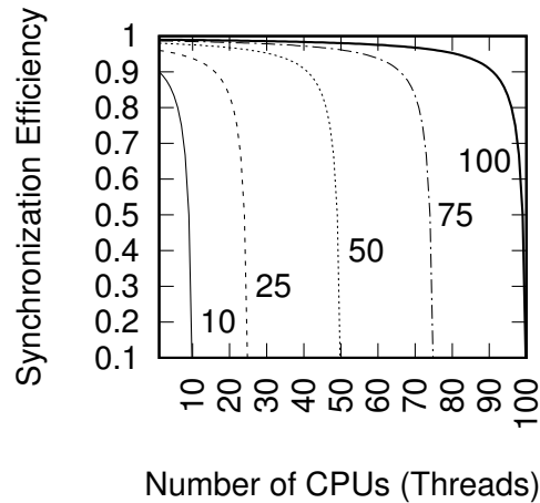
Figure 6.16: Synchronization Efficiency
