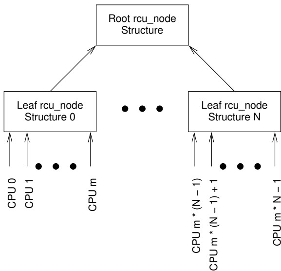
Figure 7.10: Locking Hierarchy
